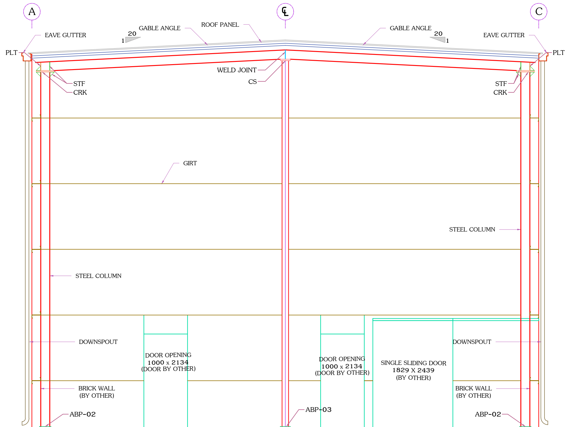
END WALL FRAMING @ GRID-1
